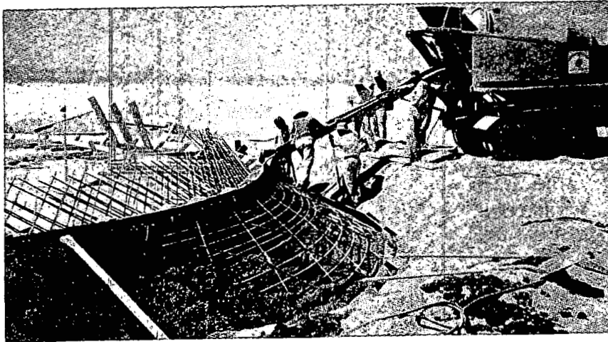
Fig. 7—Construction of foundation for responding concrete dome.
